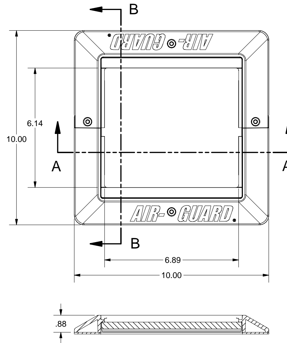
SECTION A-A SCALE 1/3
