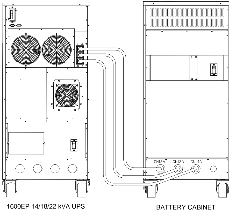
BATTERY CABINET
